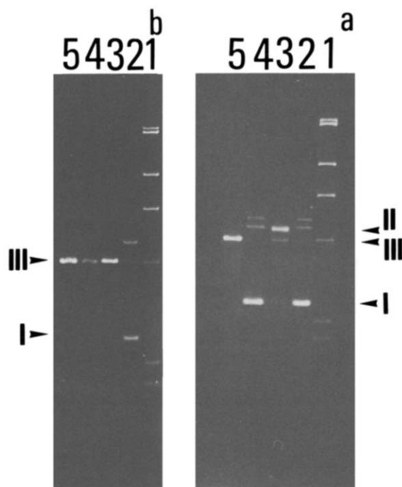
Fig.2. (a) Cleavage of supercoiled pBR322 plasmid DNA in the presence of LAHPO and (b) EcoRI digestion of pBR322 treated with LAHPO. (a) pBR322 (2.5 \mu g), LA or LAHPO (6 \mu mol) and the buffer were allowed to react at 37°C for 3 h. The reaction product was analyzed with agarose gel electrophoresis and photographed after ethidium bromide staining. Lanes: (1) marker \lambda phage DNA- HindIII digestion; (2) control pBR322 DNA; (3) LAHPO/pBR322; (4) LA/pBR322; (5) pBR322- EcoRI digestion. (b) After removal of LA or LAHPO with ethanol, DNA was digested with EcoRI (4 units) in 50 \mu l of 50 mM Tris-HCl (pH 7.6), 50 mM NaCl, 10 mM MgCl 2 at 37°C for 30 min. Lanes: (1) marker \lambda phage DNA- HindIII digestion; (2) control pBR322 DNA; (3) pBR322- EcoRI digestion; (4) LAHPO/pBR322- EcoRI digestion; (5) LA/pBR322- EcoRI digestion.
